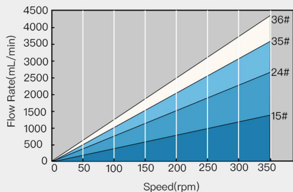
Flow Rate(0.1–350rpm)
